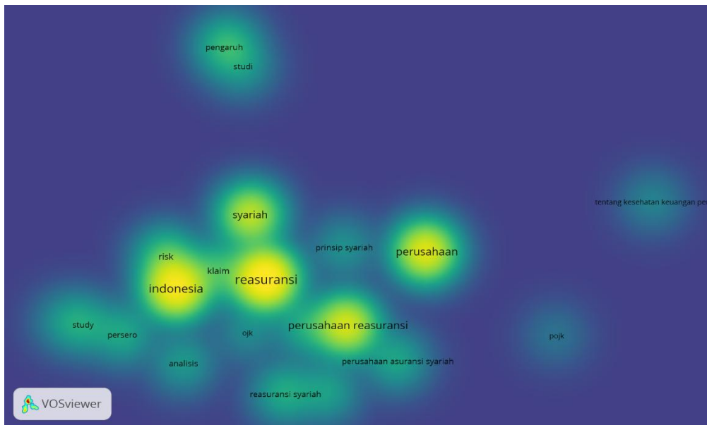
Gambar 3. Density Visualization
